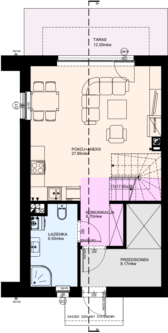
PARTER
